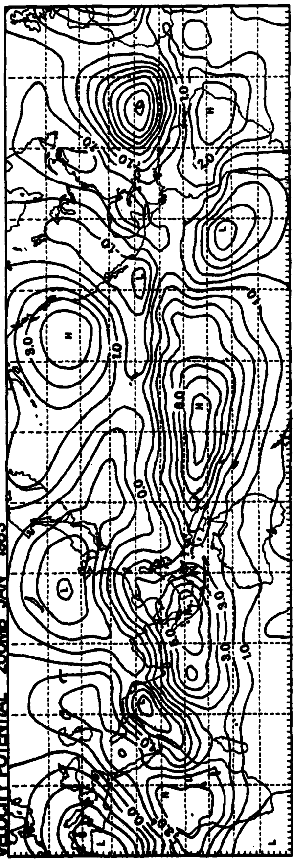
VELOCITY POTENTIAL 200MB JAN 1983
